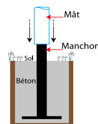
Manchon
